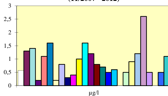
Almsee Chlorophyll-a (11/2007 - 2012)
