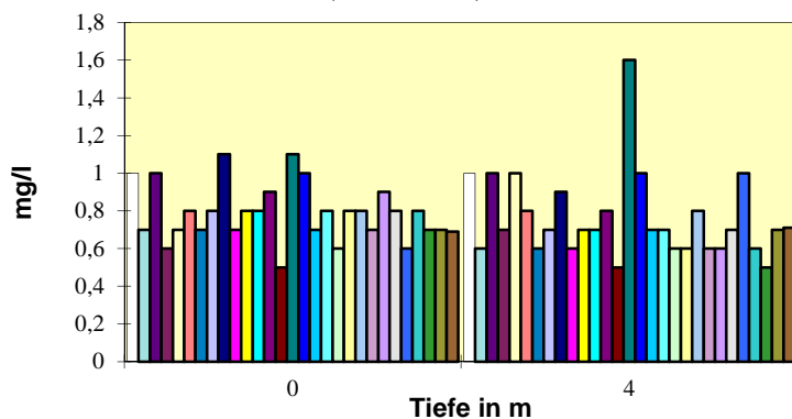
Almsee DOC (2007-2012)
