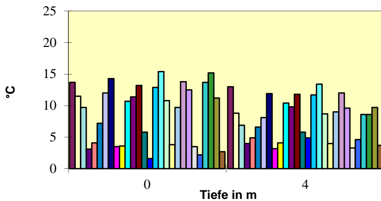
Almsee Temperatur (2007-2012)
