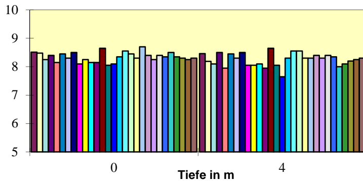
Almsee pH-Wert (2007-2012)
